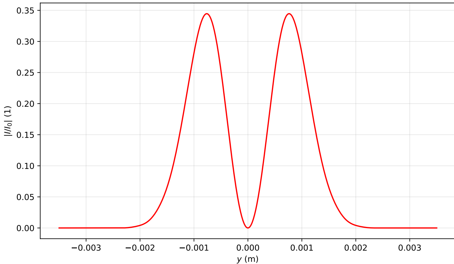
Intensity profile I(x=0, y, z=2.468)/I_0 , P_{in}=1.0P_{cr} , artificial time
